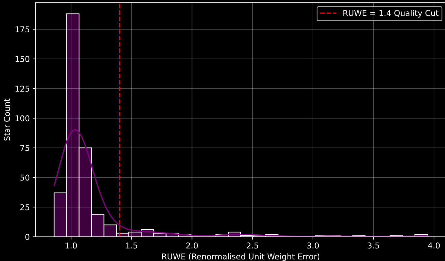
GAPOGEE DR17 Field [270+75] RUWE Distribution (n= 366)
