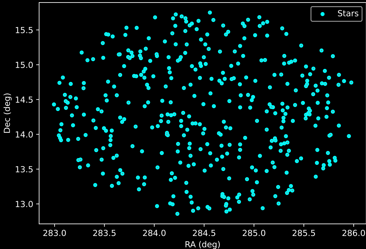
APOGEE DR17 Field: [270+75] Proper Motion Vectors for Gaia Star Field (n= 381)
