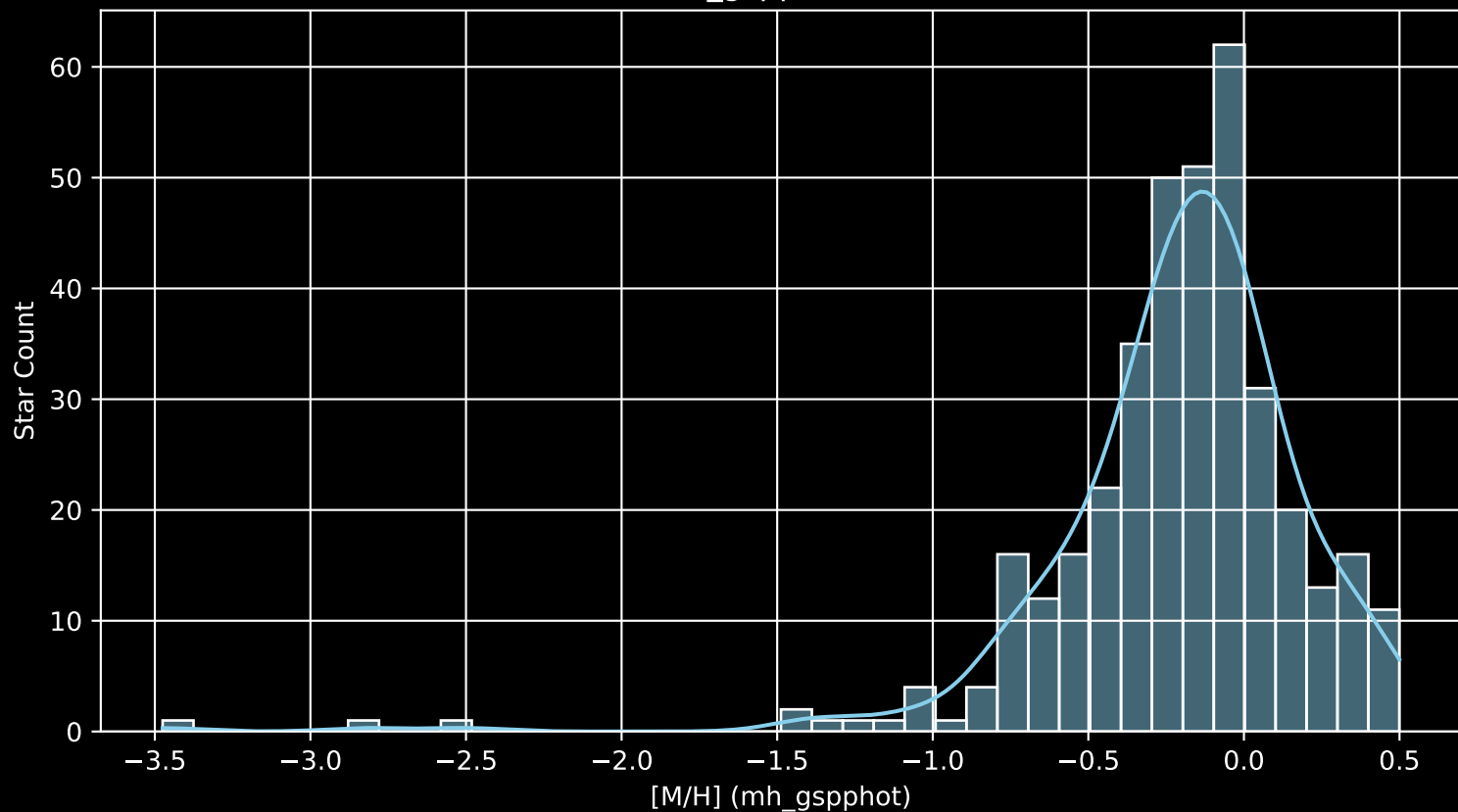
APOGEE DR17 Field: [270+75 [M/H] (mh_gspphot) (n= 372)
