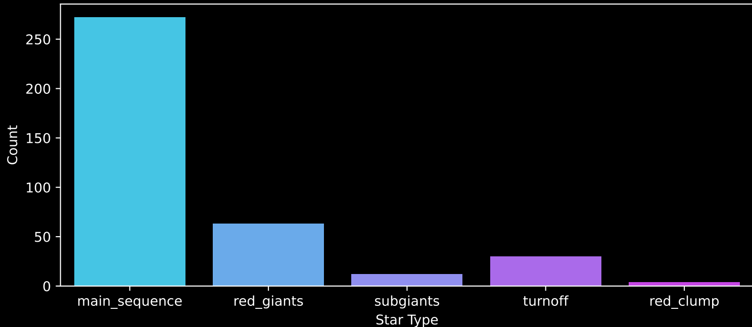
APOGEE DR17 Field: [270+75] Count plot of Star Type
