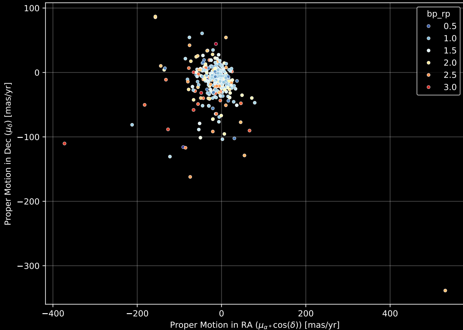
APOGEE DR17 Field: [270+75] Proper Motion Diagram (n= 381)
