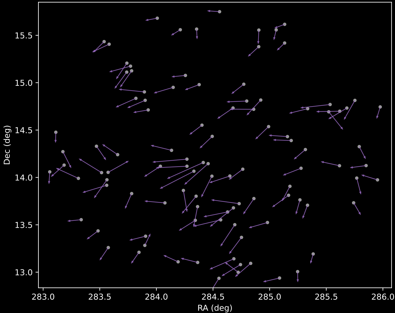
APOGEE DR17 Cluster 8 Proper Motion Vectors (n=102)
