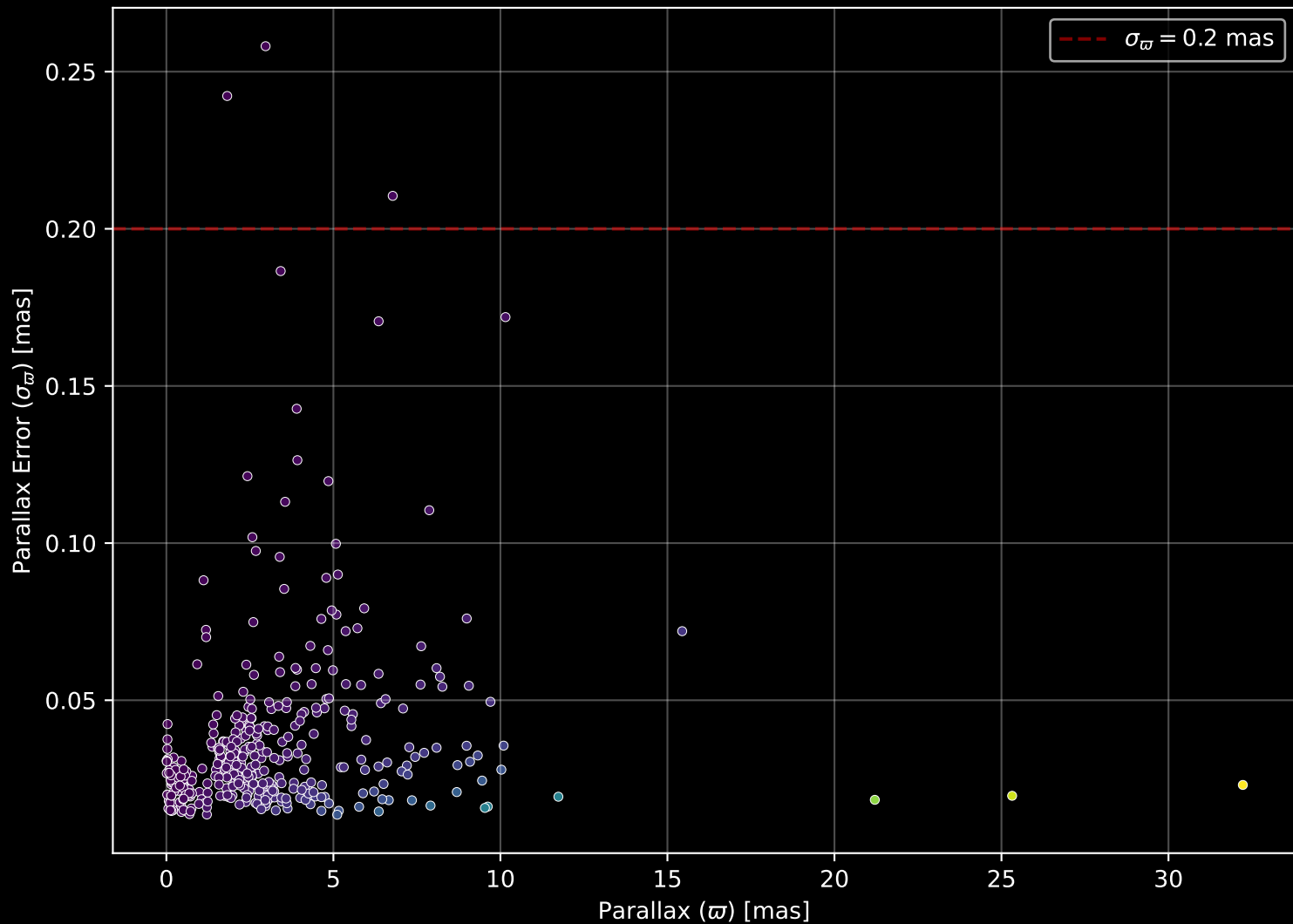
APOGEE DR17 Field: [270+75] Parallax Quality (n= 381)
