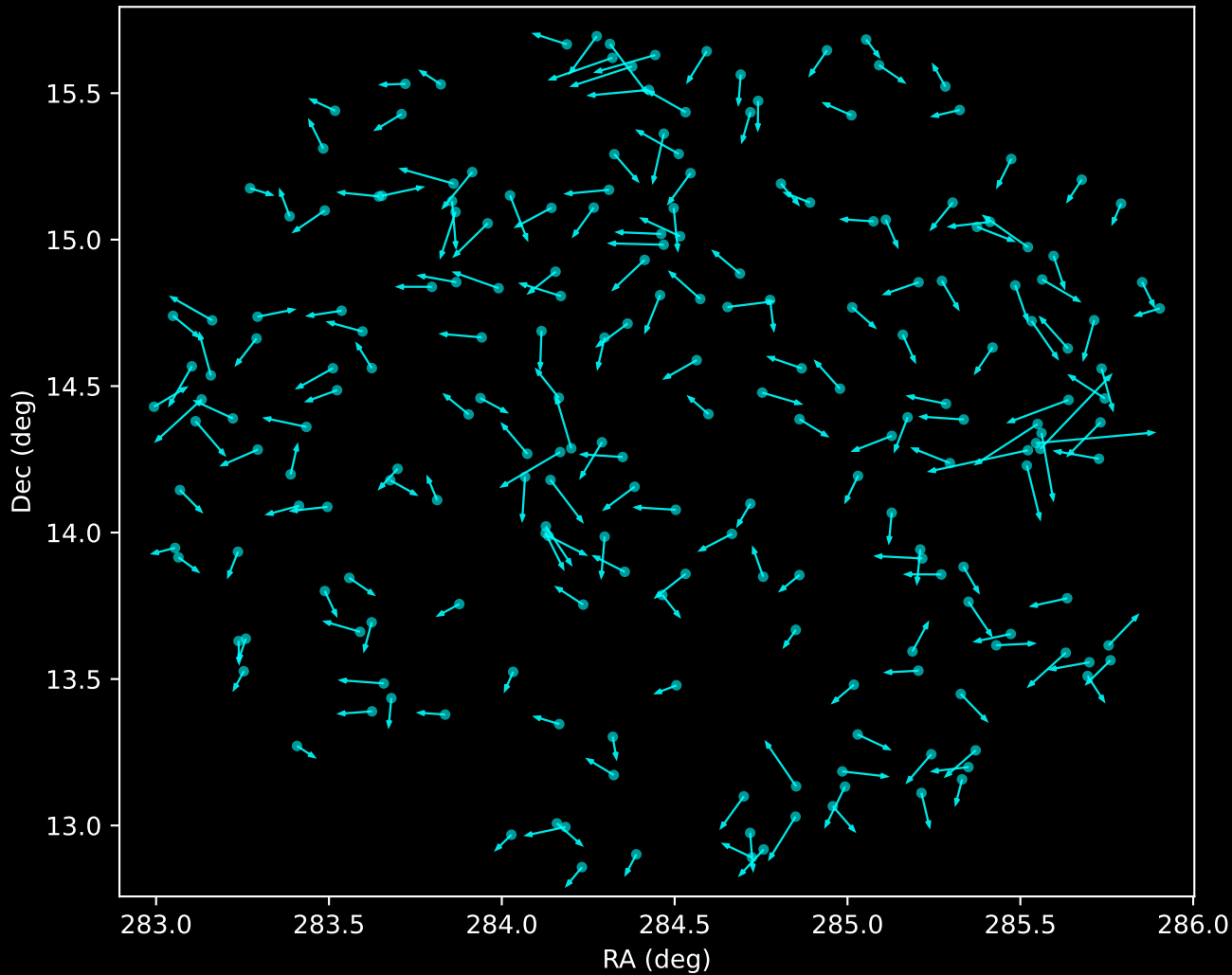
APOGEE DR17 Noise Stream Proper Motion Vectors (n=215)
